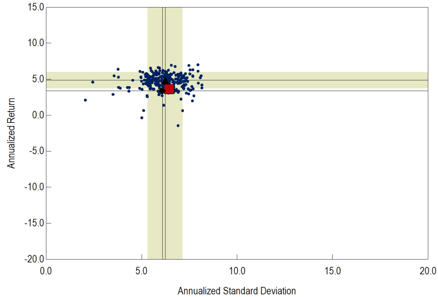
Annualized Return vs. Annualized Standard Deviation 3 Years Ending June 30, 2017
